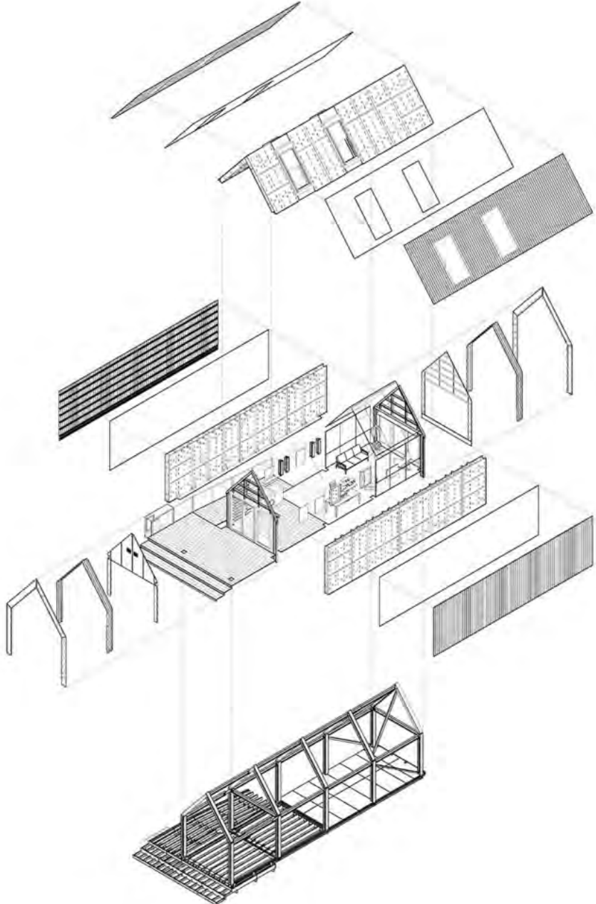
Illustrasjon: The circular building by Arup, Arup Associates
